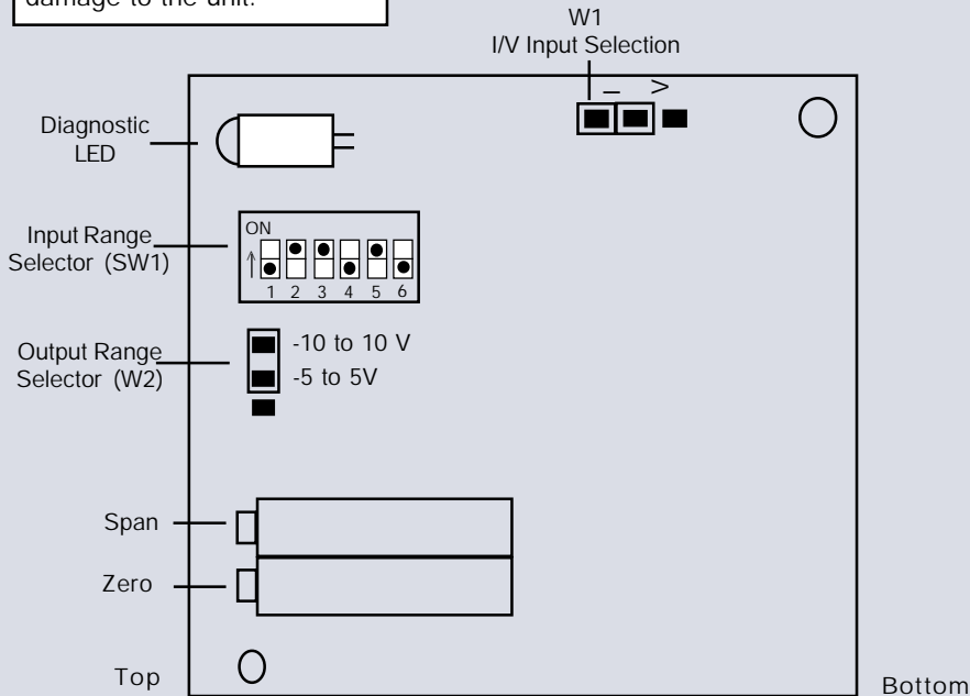
Figure 1: AP4382 I/O card factory calibration: 4-20mA input, -10 to 10V output (shown sideways to view switches)
